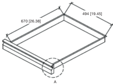
DRAWER DETAIL
